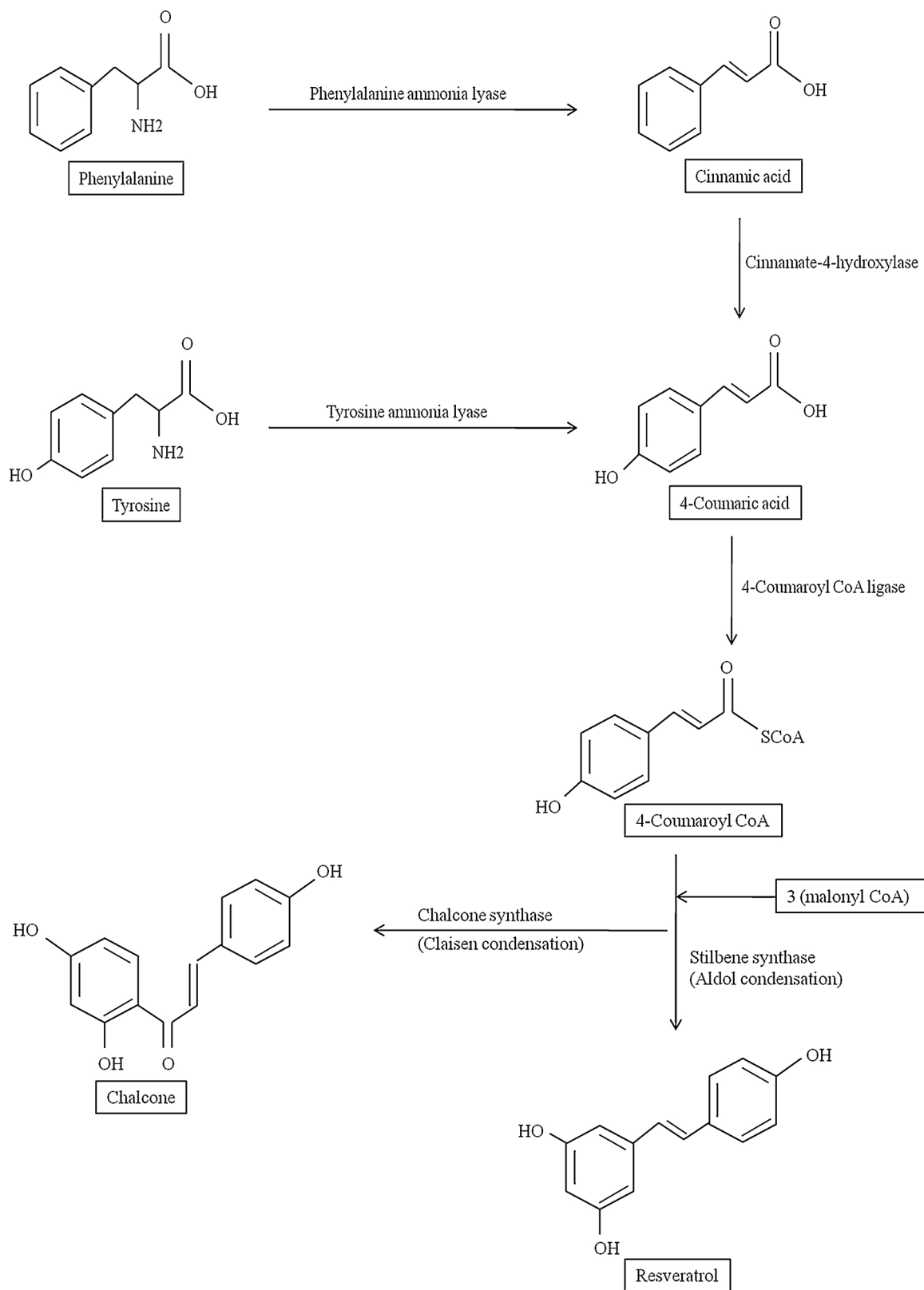
Fig. 2. Resveratrol synthesis by phenylpropanoid pathway.
