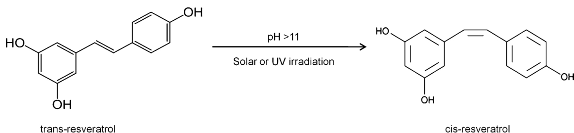
Fig. 1. pH and light induced conversion of trans to cis-resveratrol.
